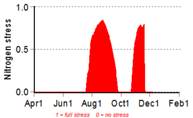
Nitrogen Stress
