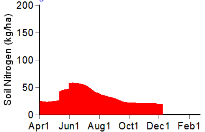
Soil Nitrogen
