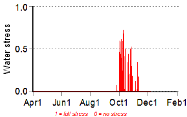
Water Stress
