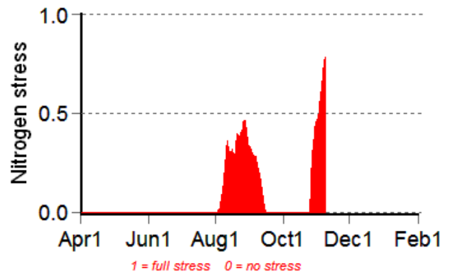
Nitrogen Stress
