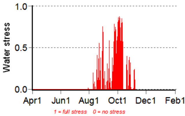
Water Stress
