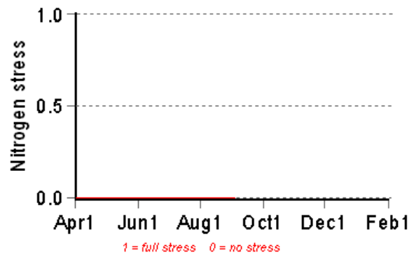
Nitrogen Stress
