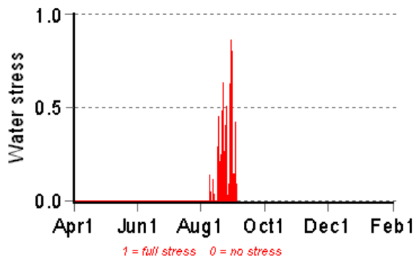
Water Stress
