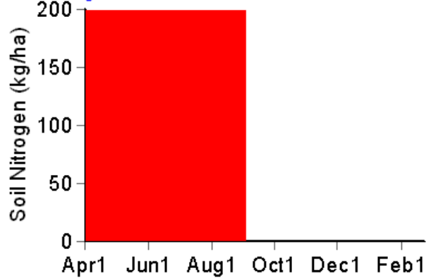
Soil Nitrogen
